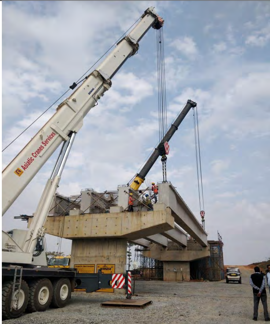
Authority Engineer Services: Girder Launching: Baharagora to Singhara (4-lane); Odisha
